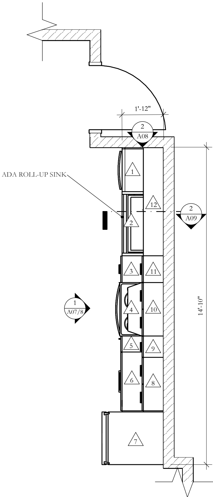
1 KITCHEN PLAN VIEW A06 3/8" = 1'-0" N
