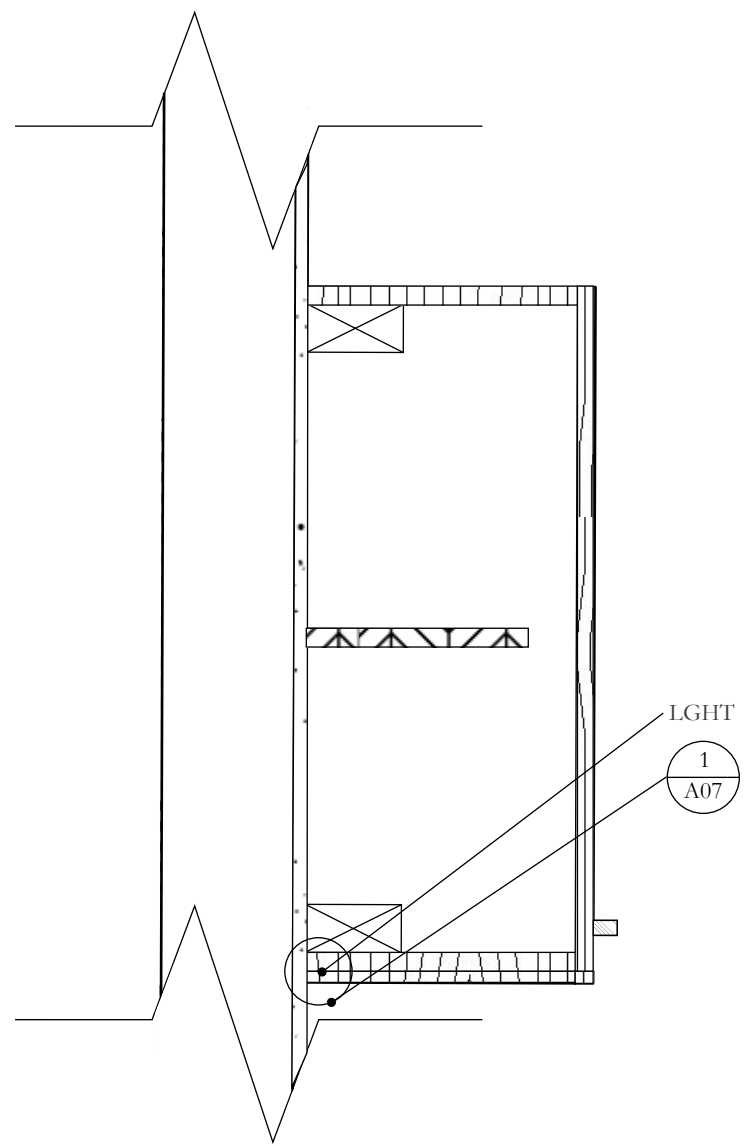
1 KITCHEN UPPER CABINET SECTION CUT A07 1 1/2" = 1'-0"
