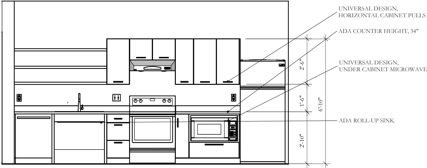
1 KITCHEN FRONT ELEVATION N A03 3/8" = 1'-0"
