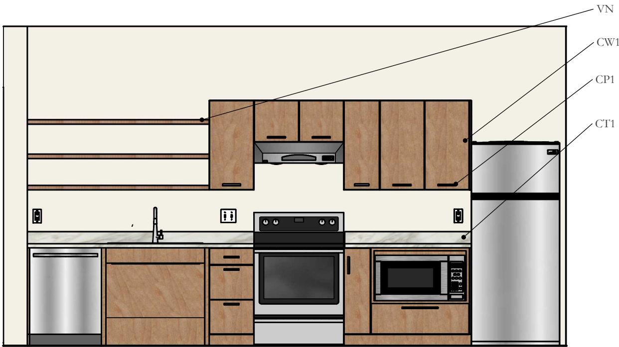
1 A03 RENDERED KITCHEN FRONT ELEVATION N 3/8" = 1'-0"
